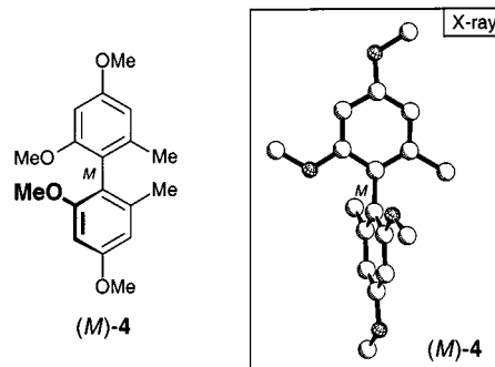
Figure 6. Crystal structure of biaryl ( M )-4
