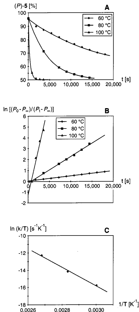
Figure 4. Determination of the atropisomerization barrier of lactone 5 : thermal racemization of ( P )- 5 in toluene (A), determination of the rate constants k (B), and Eyring plot for \Delta H^\ddagger and \Delta S^\ddagger (C)
