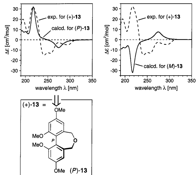
Figure 7. Determination of the absolute configuration of (+)- 13 by comparison of the experimental CD spectrum with the spectra quantum chemically calculated for ( P )- and ( M )- 13
