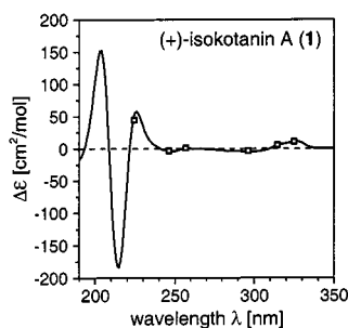
Figure 8. CD spectrum of synthetic isokotanin A ( 1 ) and comparison with literature data (marked as small squares) for “6,6'-bisiderin” [2]
