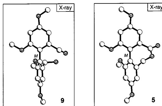
Figure 3. Crystal structures of compounds 5 and 9
